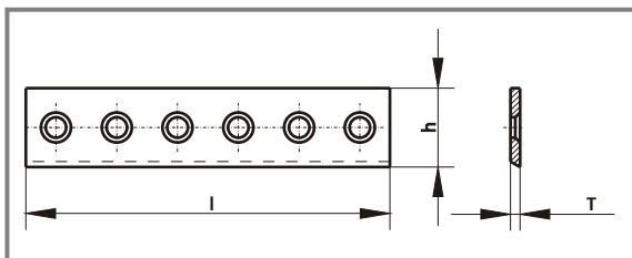
LT-1 Single row steel strips
