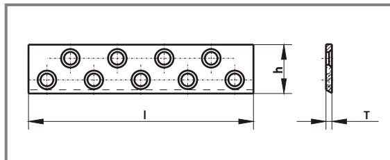
LT-2 Double row steel strips
